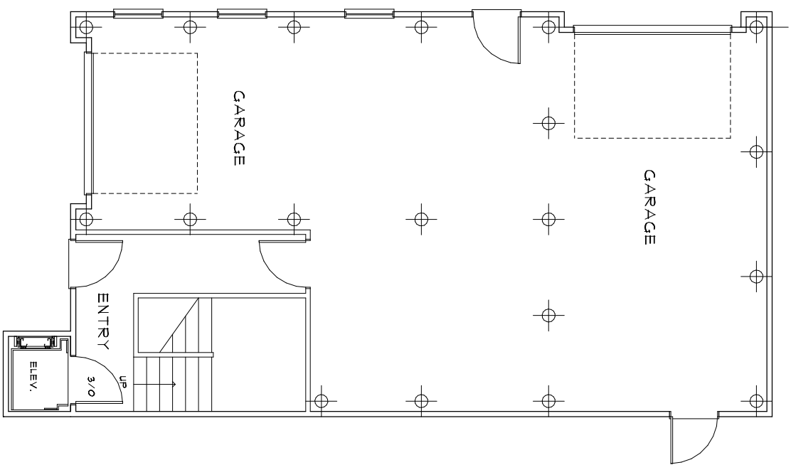
GROUND LEVEL PLAN 1/4" = 1'-0" COMMON
